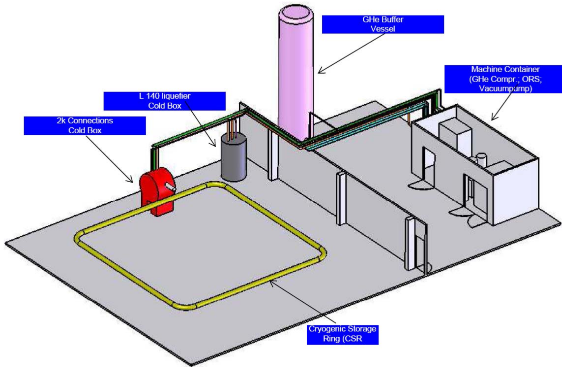
Cooling System for the Cryogenic Storage Ring CRS
