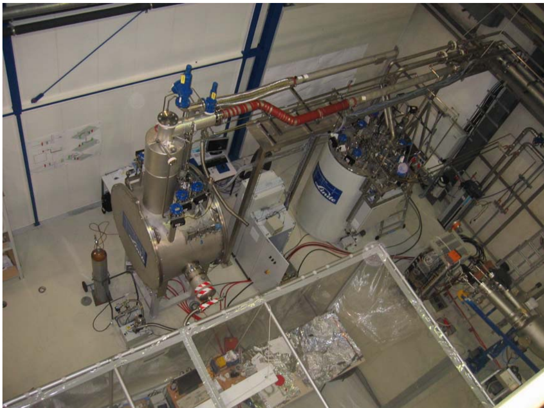
Liquefier Coldbox and 2K Connection Coldbox
